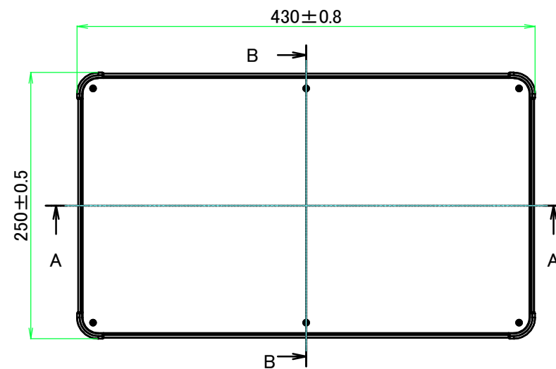
E view
